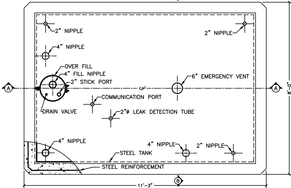
PLAN VIEW
