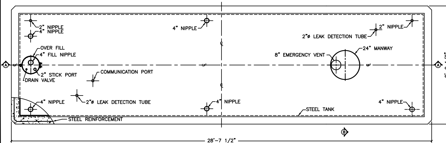
PLAN VIEW
