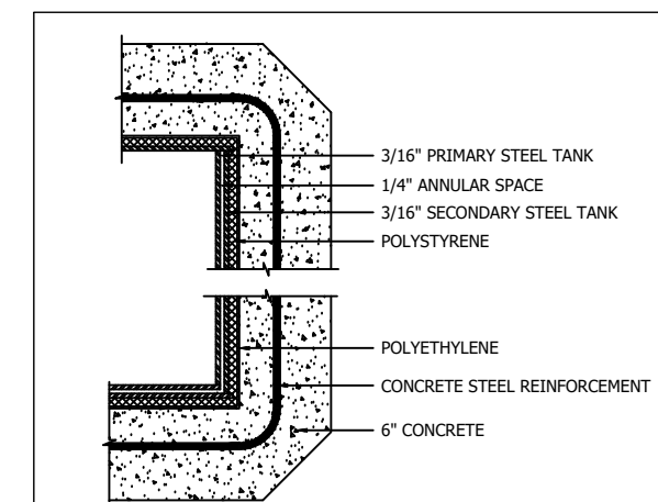
2 CORNER DETAILS
