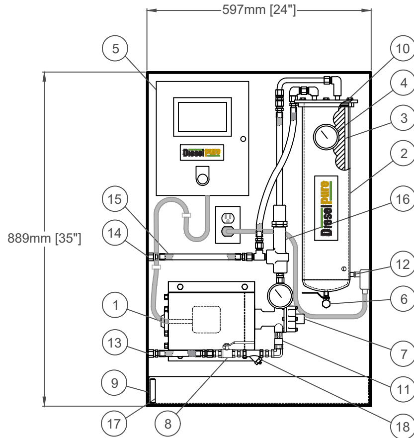
FRONT VIEW
