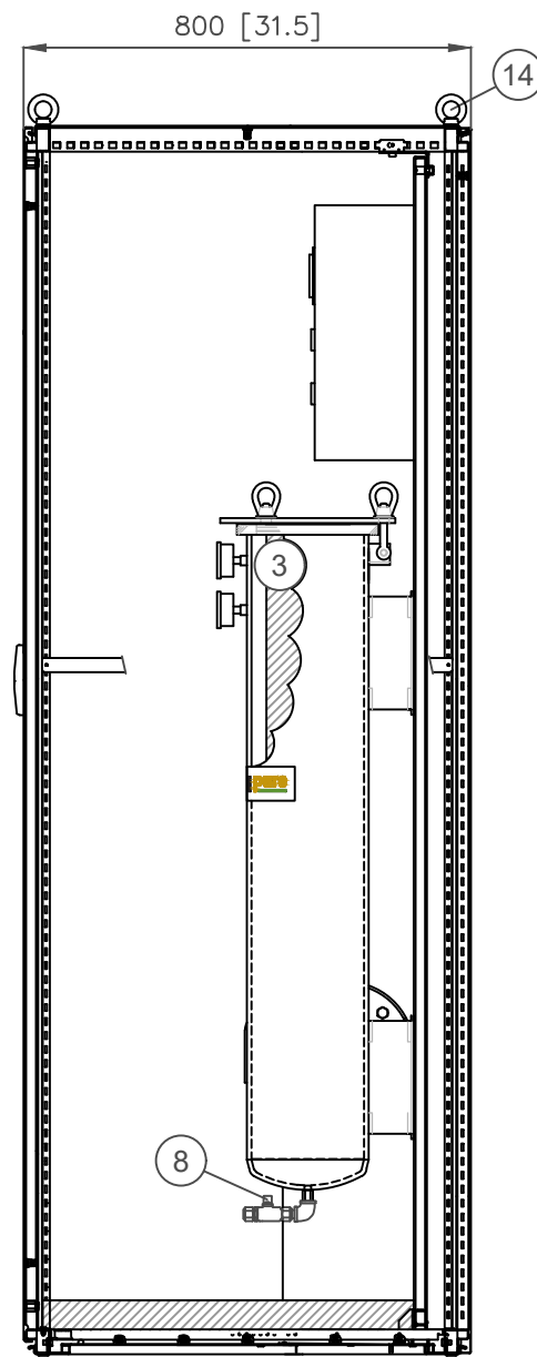
RIGHT-SIDE VIEW
