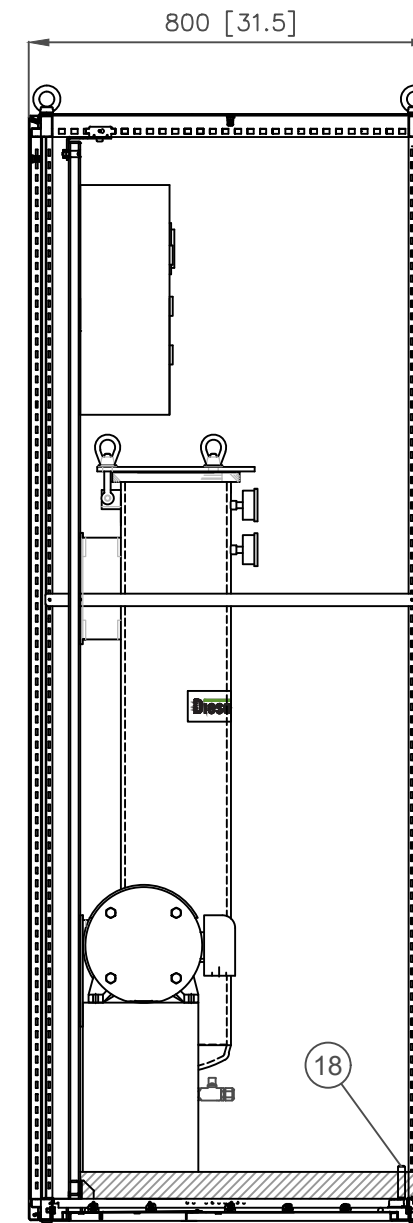
LEFT-SIDE VIEW
