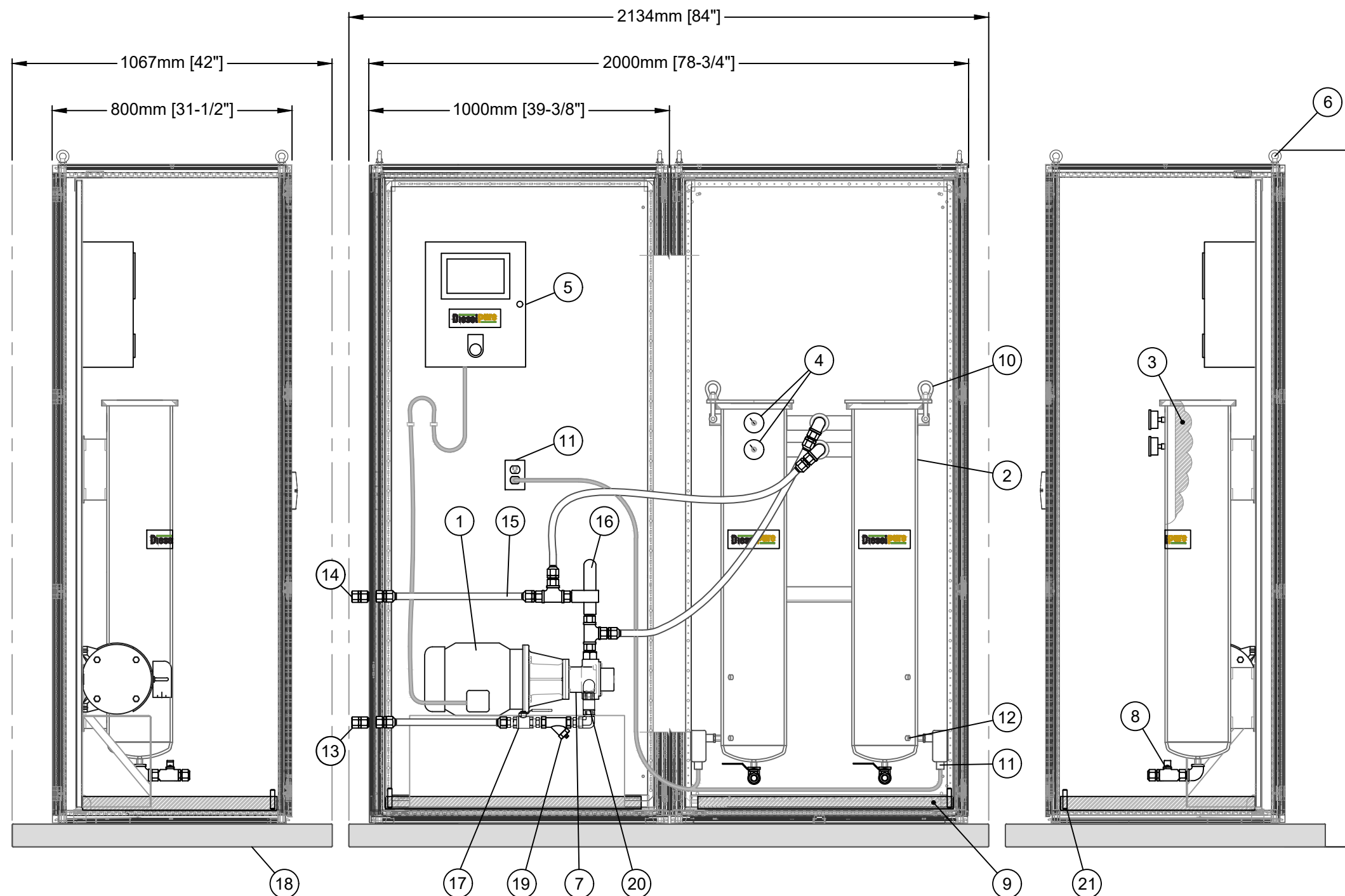
LEFT-SIDE VIEW
